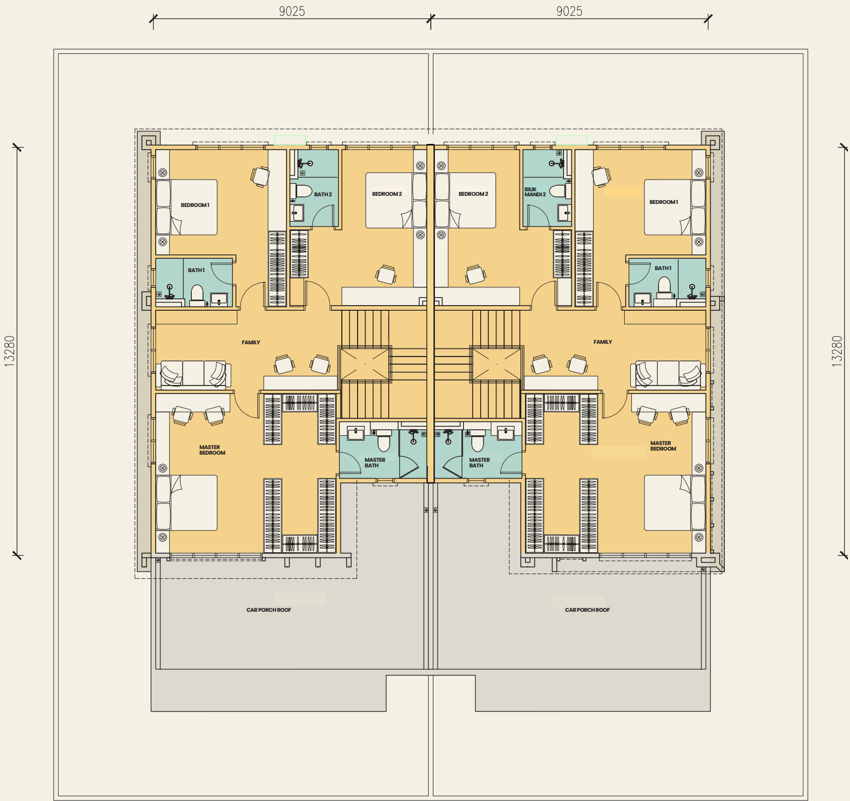
First Floor
