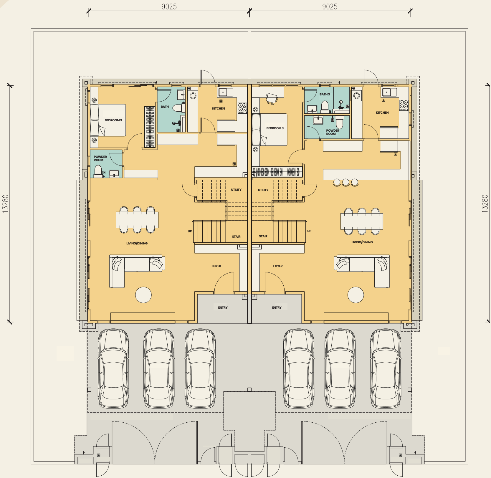
Ground Floor
