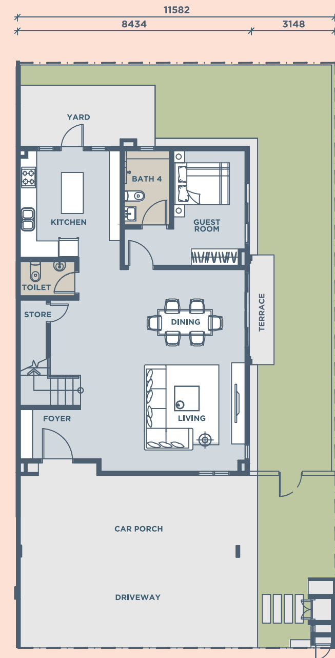
GROUND FLOOR
