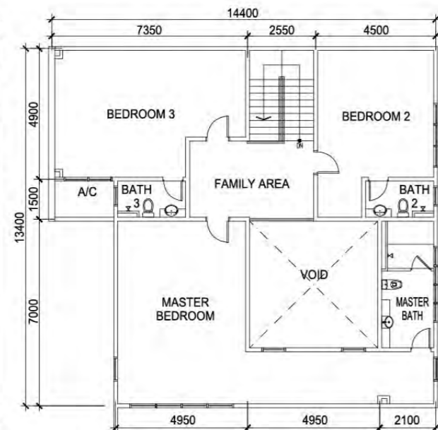
TYPE PH2 UPPER FLOOR
