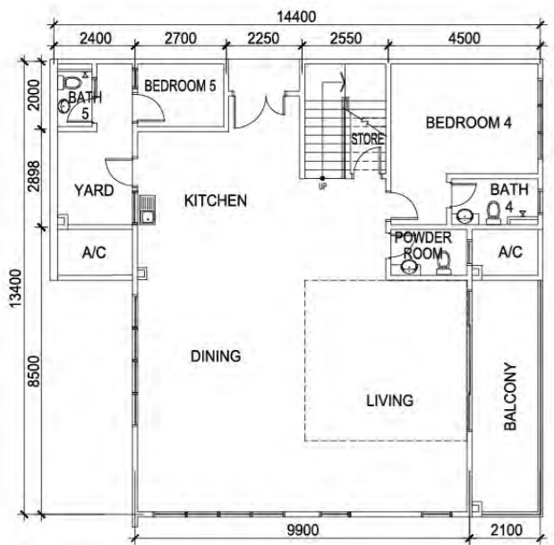
TYPE PH2 LOWER FLOOR
