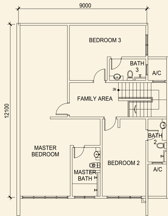
TYPE PH1 UPPER FLOOR
