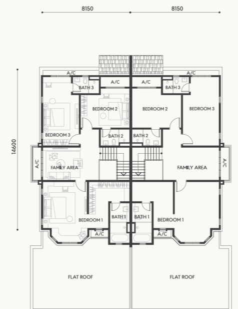
TYPE 3B - FIRST FLOOR
