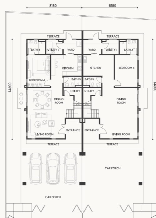
TYPE 3B - GROUND FLOOR
