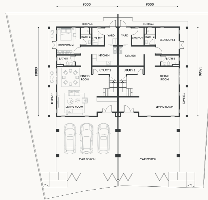
TYPE 3A - GROUND FLOOR
